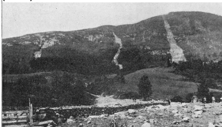
Fig. 3.9.3. Landslide scars on Mt. Greylock 1901 (top) and 1999 (bottom)
