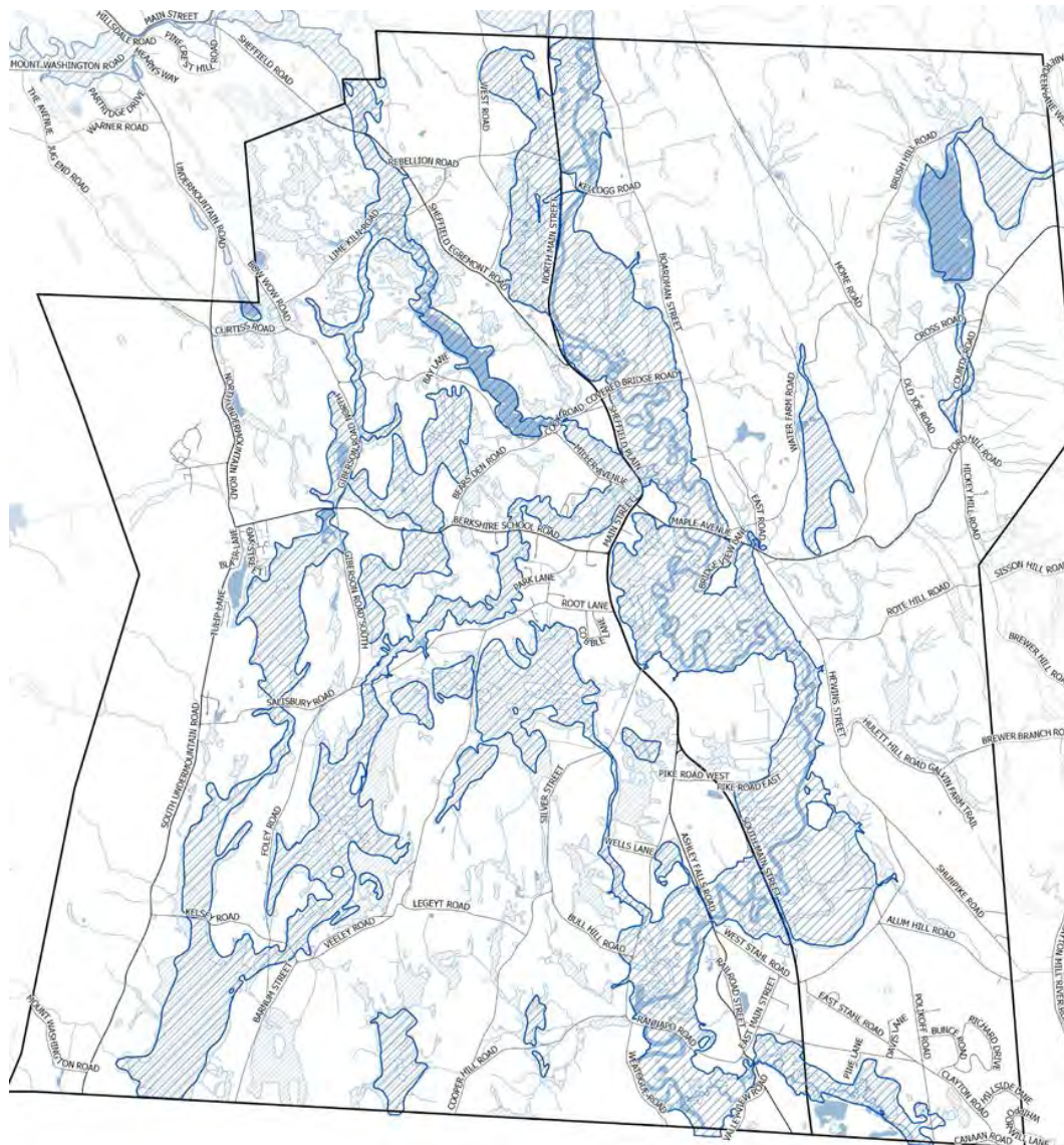
Fig. 3.2.5. 100-yr Floodplain Areas (Blue hatching)
