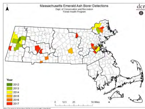
Fig. 3.8.4. Emerald Ash Borer Dispersal 2017
