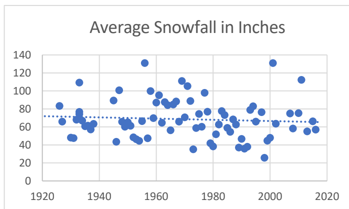
Figure 3.6.1. Average Snowfall in Berkshire County
