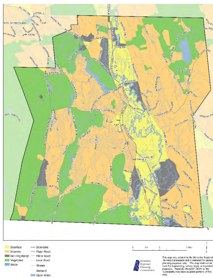
Fig. 3.8.2. SILVUS Wildland-Urban Interface Map
