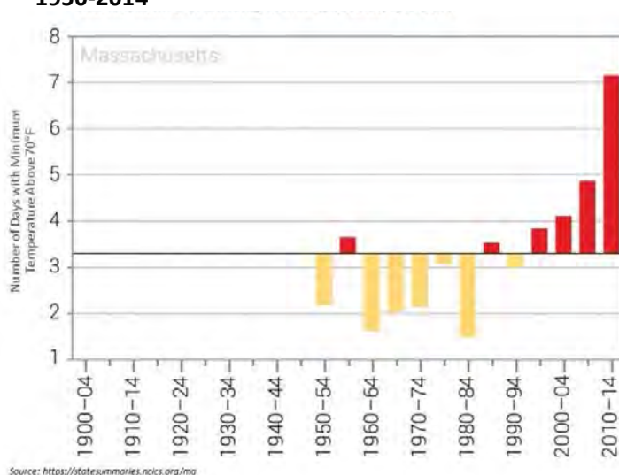
Fig. 3.4.8. Observed Number of Warm Nights in MA 1950-2014
