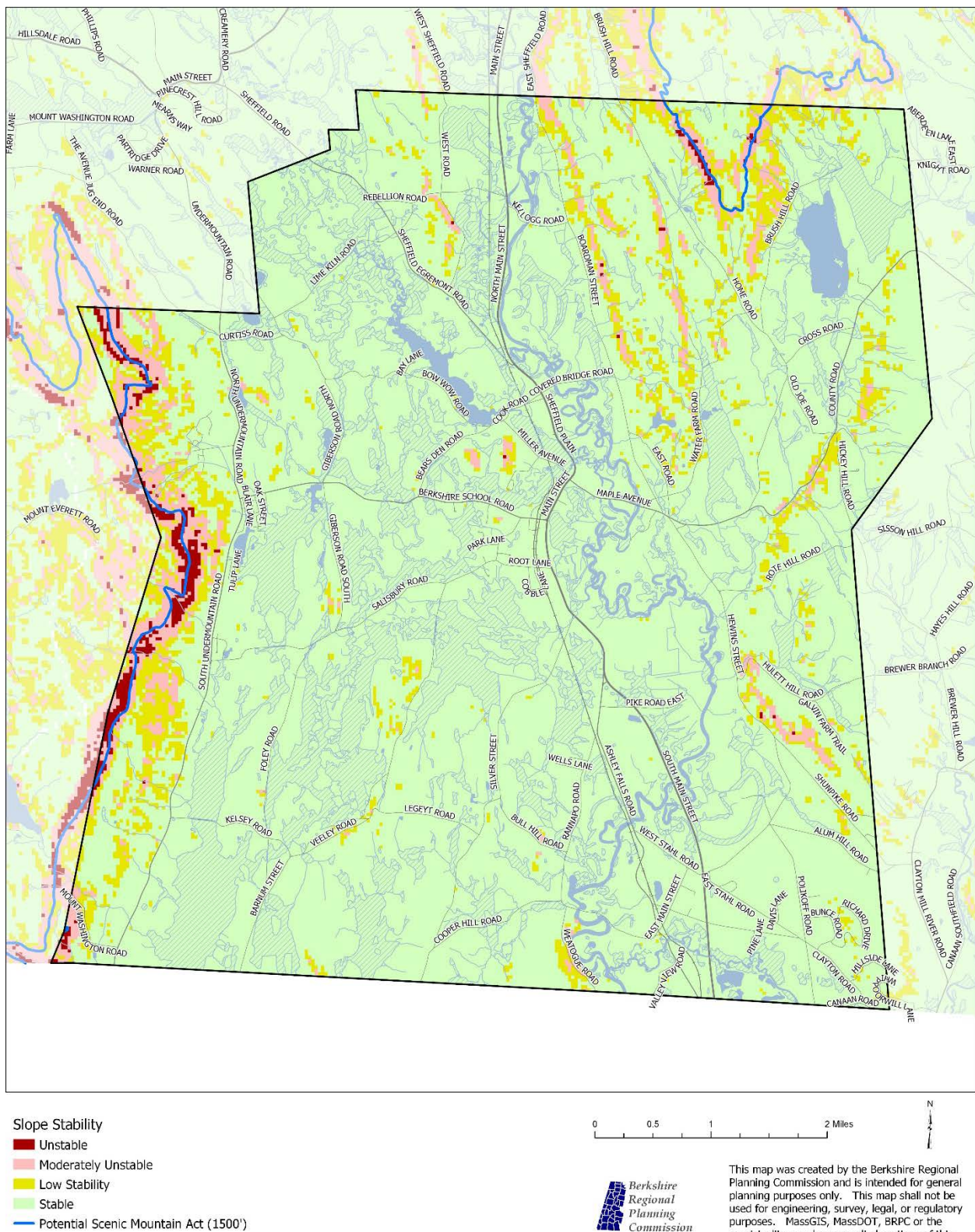
Fig. 3.9.2. Slope Stability (using the Massachusetts Geologic Survey) and Potential Berkshire Scenic Mountain Act Boundaries
