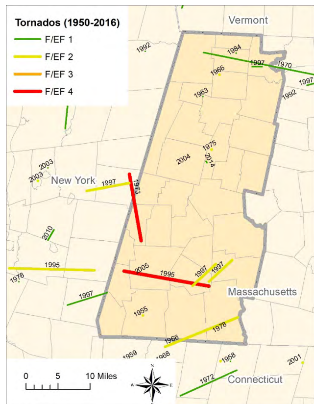
Fig. 3.4.3. Tornadoes in the Berkshire Region and Severity
