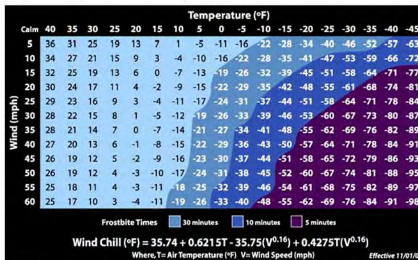
Fig. 3.4.6. Wind Chill Temperature Index and Frostbite Risk
