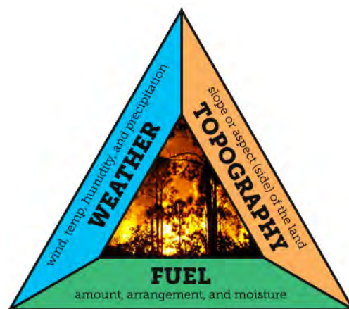
Fig. 3.8.1. Fire Behavior Triangle
