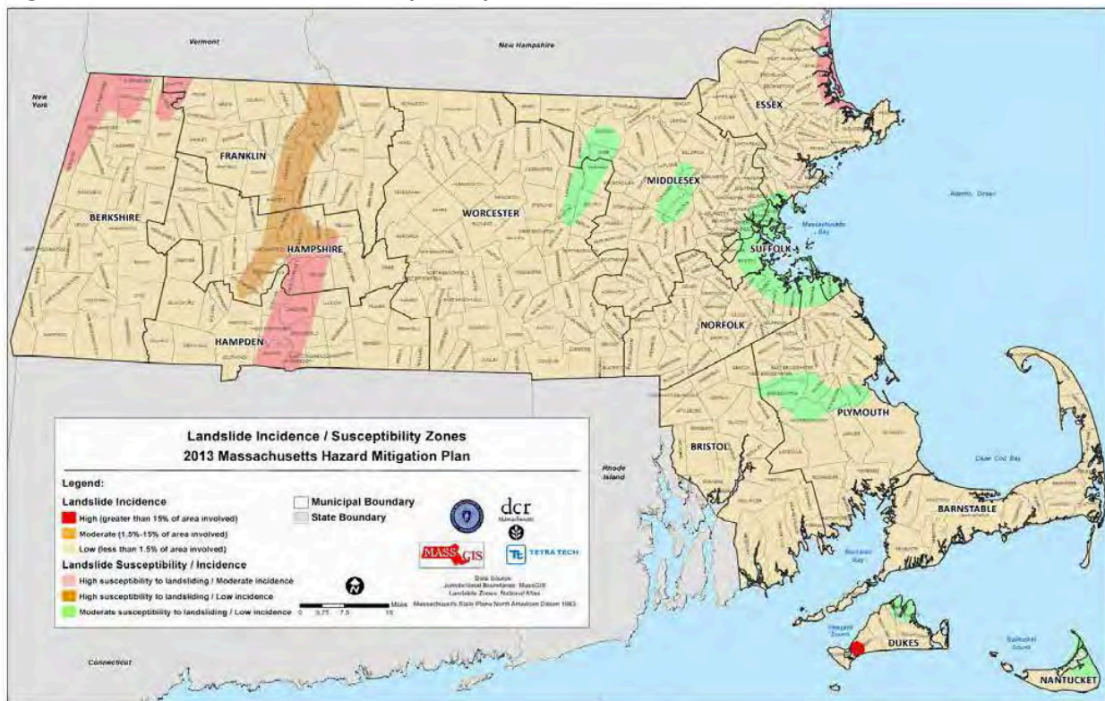
Fig. 3.9.1 Landslide Incidence / Susceptibility Zones
