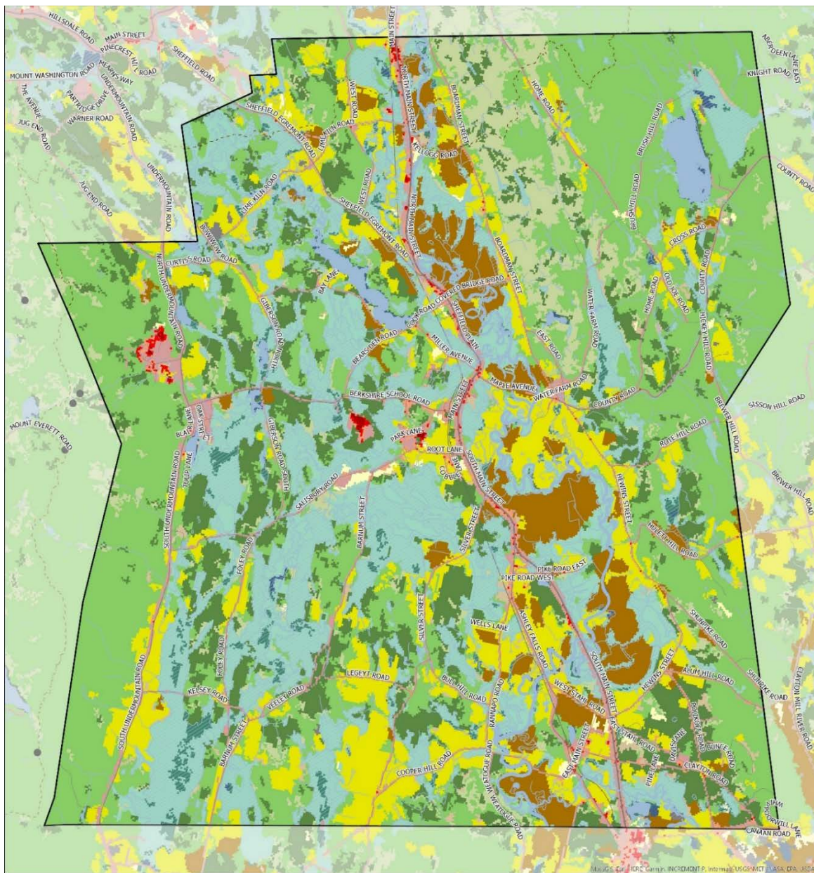
Fig. 3.8.3. Developed Areas (Red, Pink) – National Land Cover Data for Sheffield
