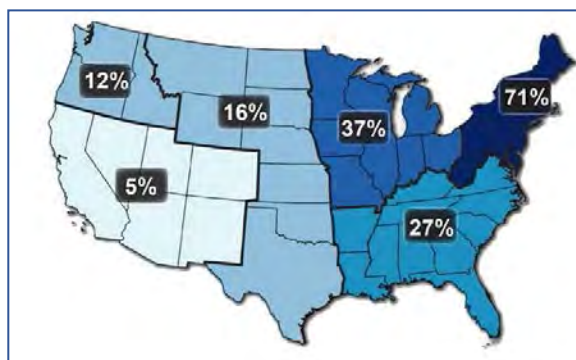
Fig. 3.2.2. Increase in Precipitation Falling in Top 1% Extreme Precipitation Events 1958-2012
