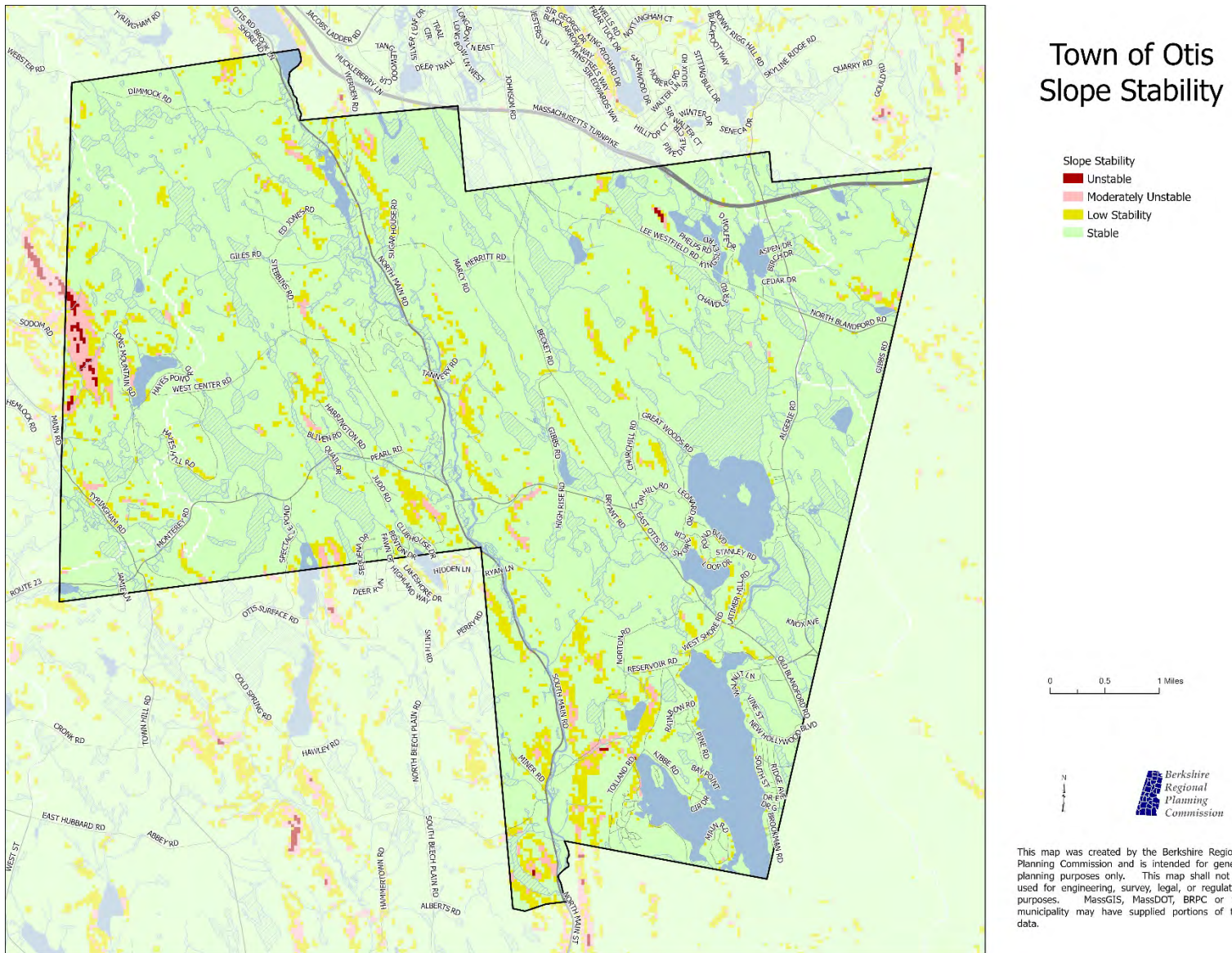
Figure 3.44. Slope Stability Map
