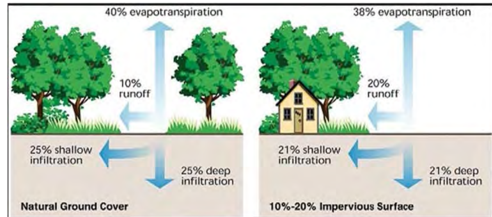
Fig. 3.12. Stormwater runoff doubles in modest development
