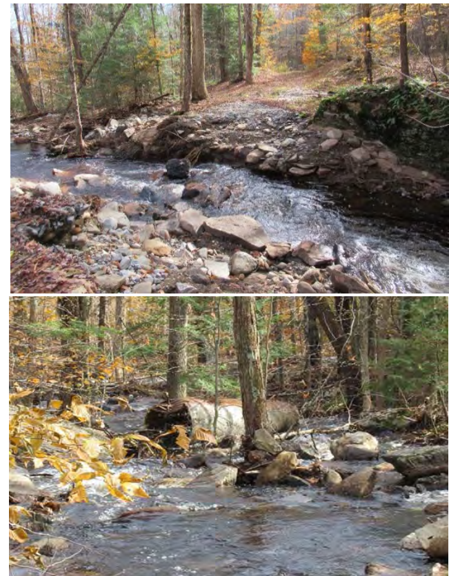
Figs. 3.7 & 3.8. Top: Stebbins Rd. damage at Cone Brook crossing due to beaver dam breach; Bottom: Stebbins Rd. culvert washed downstream
