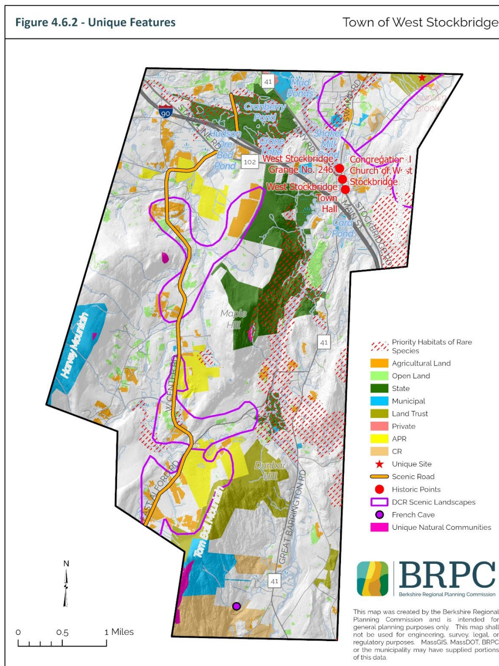
Fig. 4.9. Unique Features
