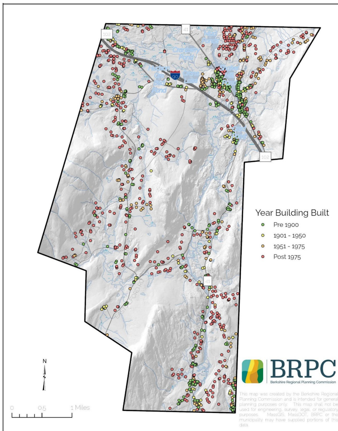
Fig.3.6. Development Trends
