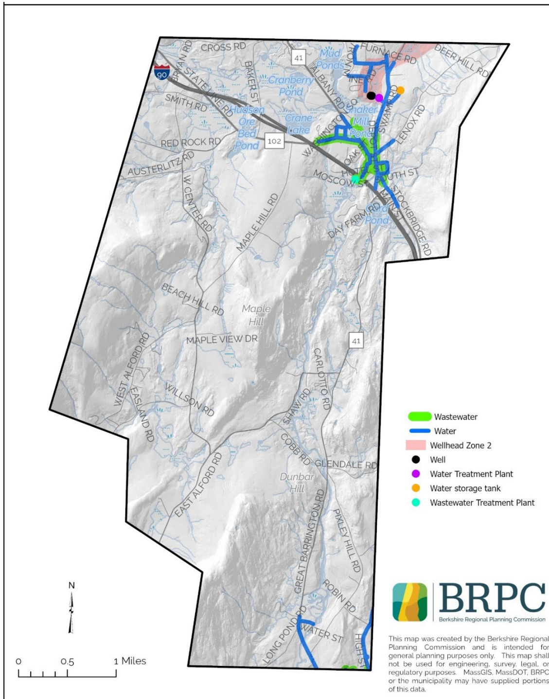
Fig. 3.4. Municipal Water and Sewer Infrastructure
