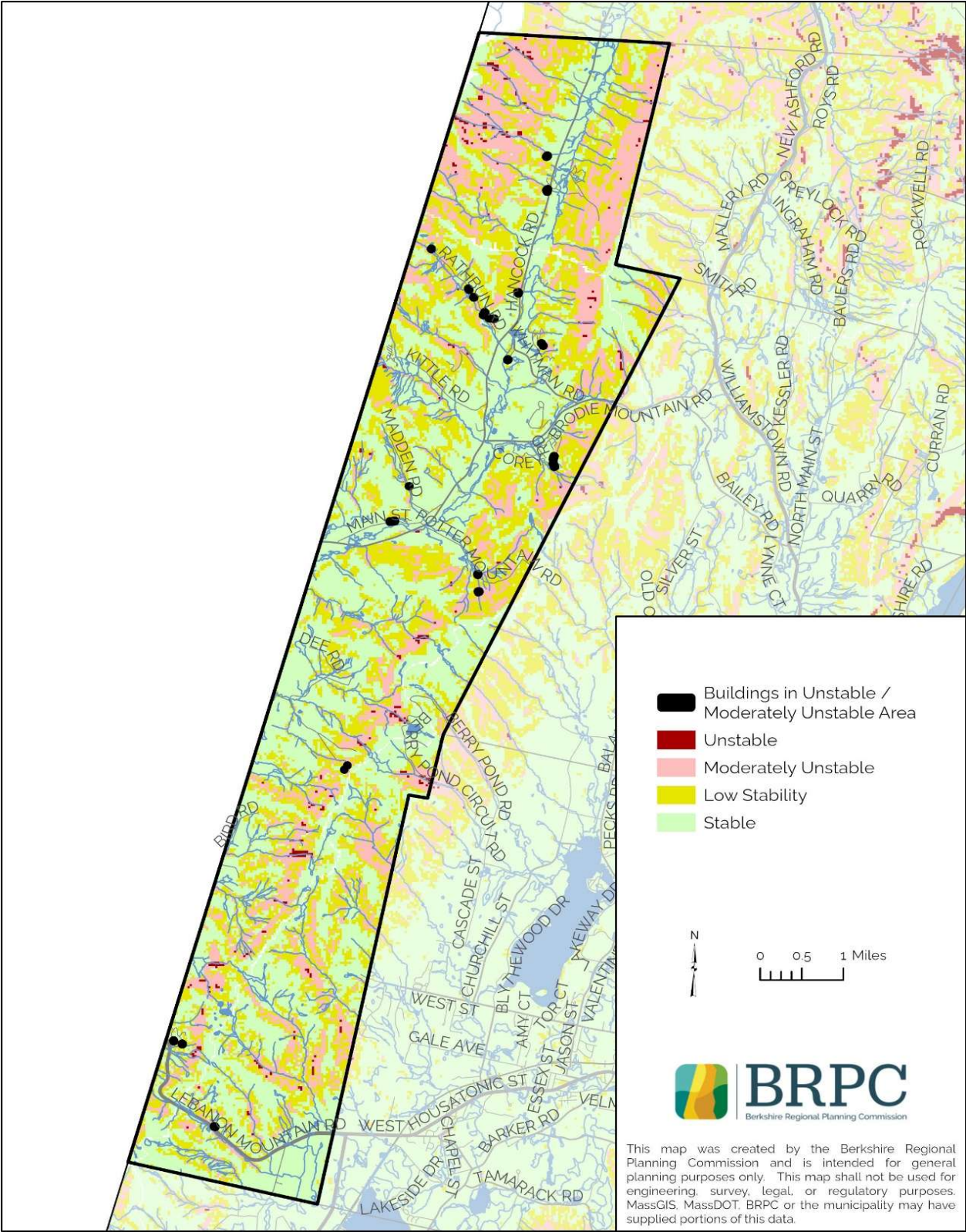
Figure 3.24 Town of Hancock Slope Stability Map
